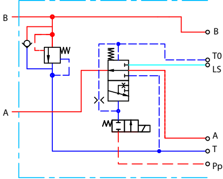
Multi-valve schematic
